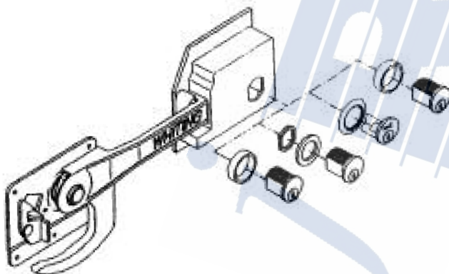
77 type lock with lockable keeper for Dry Freight & Excel 2000 TempSaver range & Continental II & III Lock cylinders available: Yale, Best, Assa & Abloy
